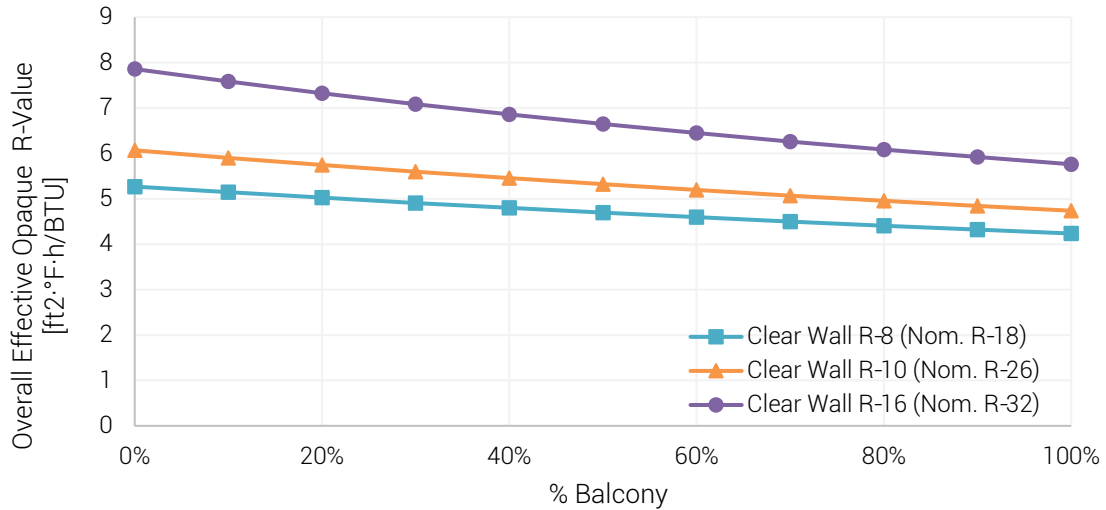
Figure 9 - Impact of Balcony on Thermal Performance
