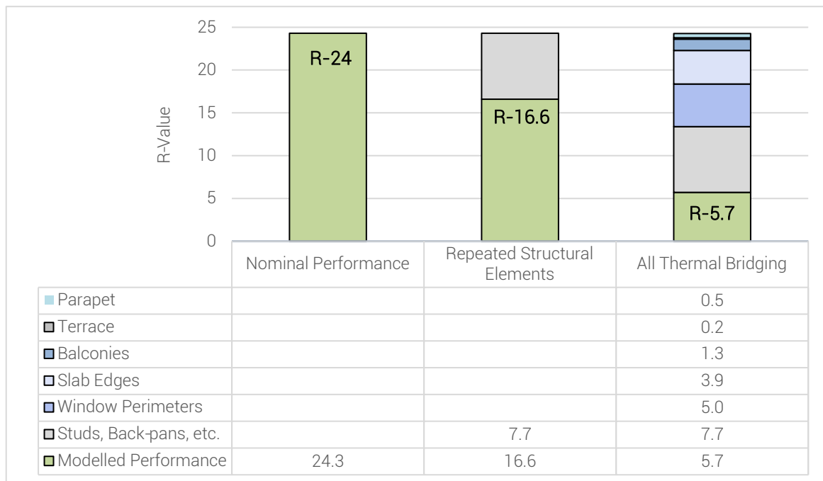
Figure 7 - Impact of Thermal Bridging on Opaque Envelope Performance 7
