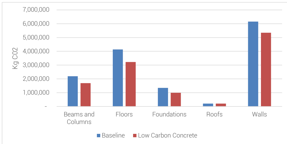
Figure 19 – Low Carbon Concrete – 30-40% SCM and GUL
